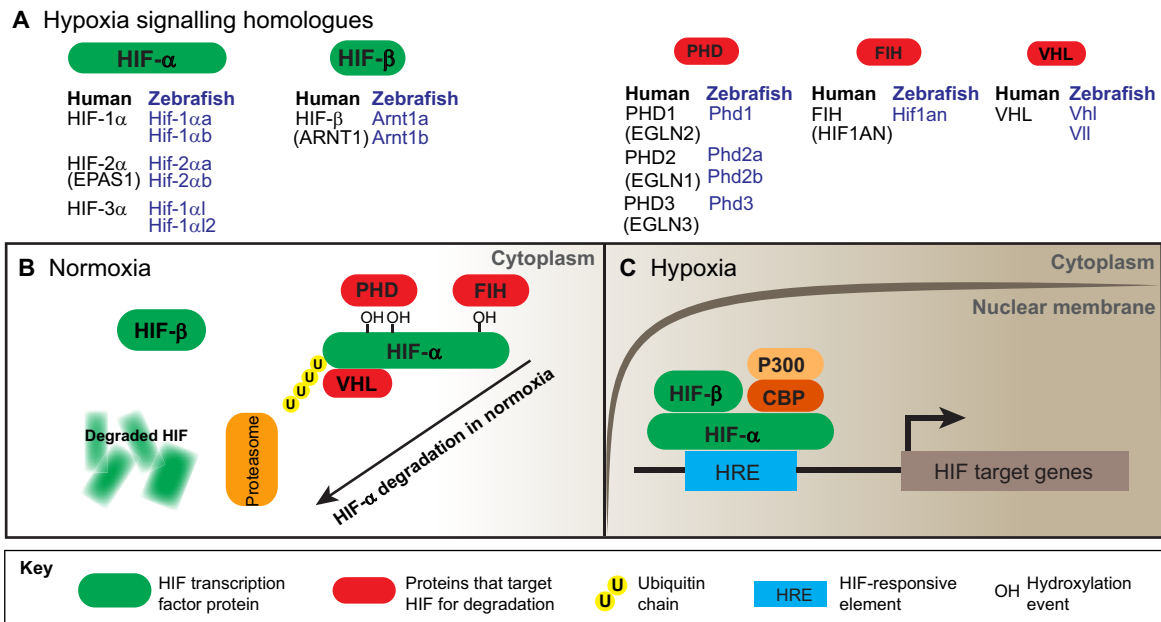
Fig. 1. Schematic diagram of the HIF-signalling system and zebrafish homologues. (A) Proteins of the HIF-signalling pathway are illustrated, with HIF proteins in green and proteins that target HIF for degradation in red. The human isoforms are listed, with their zebrafish counterparts in blue text. (B) In normoxia, the hydroxylase enzyme PHD and the VHL protein target HIF-α for ubiquitination in the cytoplasm and subsequent degradation by the proteasome. A second hydroxylase enzyme, FIH, hydroxylates a C-terminal asparagine residue on HIF-α in normoxia to repress the transactivation function of HIF. (C) In hypoxia, hydroxylase enzymes are silenced, and HIF translocates to the nucleus and binds its cofactors, where it upregulates target gene expression by binding to HREs in their regulatory regions. Abbreviations: CBP, CREB-binding protein; FIH, factor inhibiting HIF; HIF, hypoxia-inducible factor; HREs, HIF-responsive elements; P300, E1A binding protein; PHD, prolyl hydroxylase domain-containing proteins; VHL, von Hippel-Lindau.
