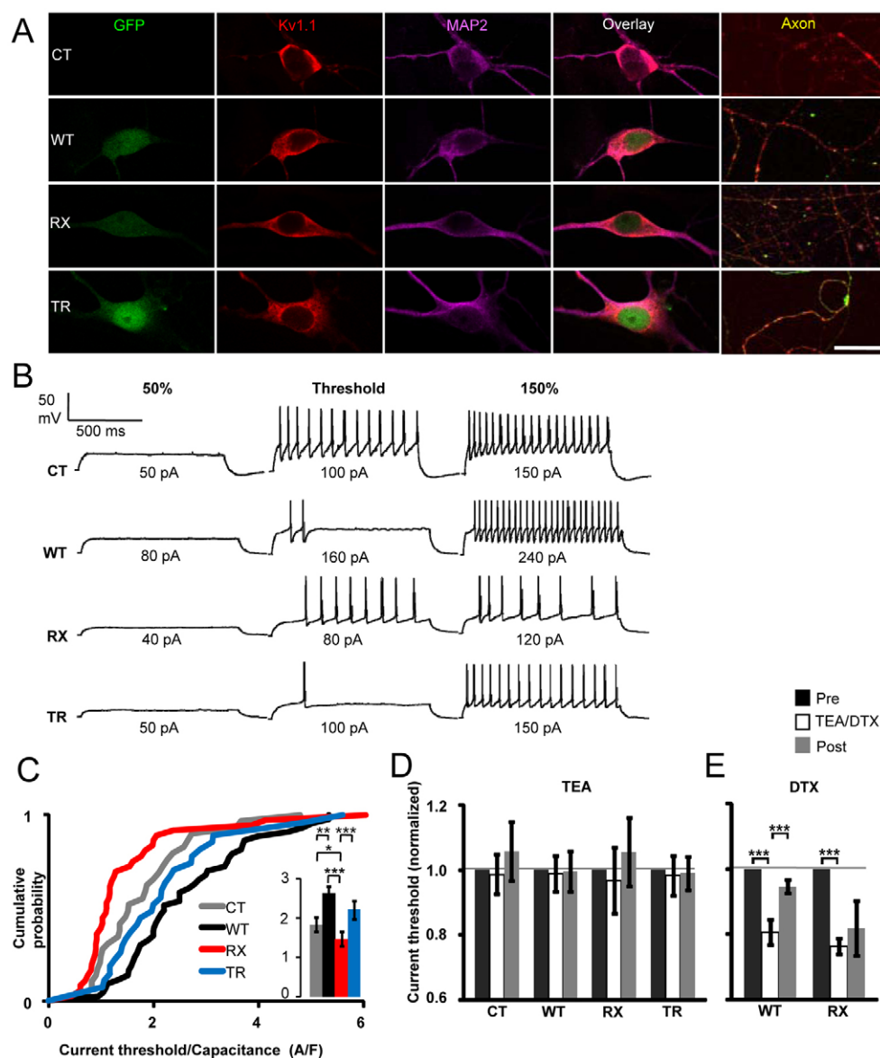
Fig. 1. Kv1.1 manipulation affects excitability. (A) Lentiviral expression of Kv1.1 does not alter overall Kv1.1 distribution in neurons after 15 days in vitro. CT, WT, RX and TR neurons stained for Kv1.1 (red, second column) and the dendrite marker microtubule associated protein 2 (MAP2) (magenta, third column). Transduction was verified by green fluorescent protein (GFP) expression (first column), which was driven by a separate promoter. Kv1.1 was primarily present in the perikaryal and somato-dendritic compartments but was also found in axons (defined by the absence of MAP2 staining, fifth column). Aggregation of endogenous Kv1.1 in the endoplasmic reticulum (ER) was not observed in any group. Bar, 25 \mu m (somato-dendritic panels), 120 \mu m (axonal panels). (B) WT and RX Kv1.1 have opposite effects on neuronal excitability. Example traces from CT neurons and neurons expressing WT, RX and TR Kv1.1 at 50%, 100% and 150% of the current threshold. The scale bar applies to all traces. (C) Cumulative probability plot showing an increase in the current threshold (normalized by capacitance) for neurons expressing WT Kv1.1 (black, n=43 ) compared with CT neurons (gray, n=29 ), and a reduction in the current threshold for RX-expressing neurons (red, n=36 ) compared with CT, WT and TR (blue, n=27 ) neurons. Inset: mean \pm s.e.m. current threshold/capacitance (using the same color code), based on the results of the Mann-Whitney U -test (* P \leq 0.05 , ** P \leq 0.01 , *** P \leq 0.001 ). (D) TEA (1 mM) had no consistent effect on the current threshold in any group. (E) \alpha -DTX (100 nM) reduced the current threshold (normalized by capacitance) in both WT- and RX-expressing neurons (paired t -tests).
