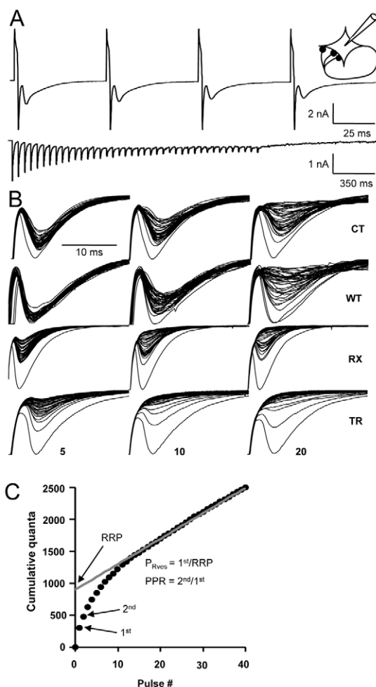
Fig. 3. Effects of Kv1.1 manipulation on neurotransmitter release.
